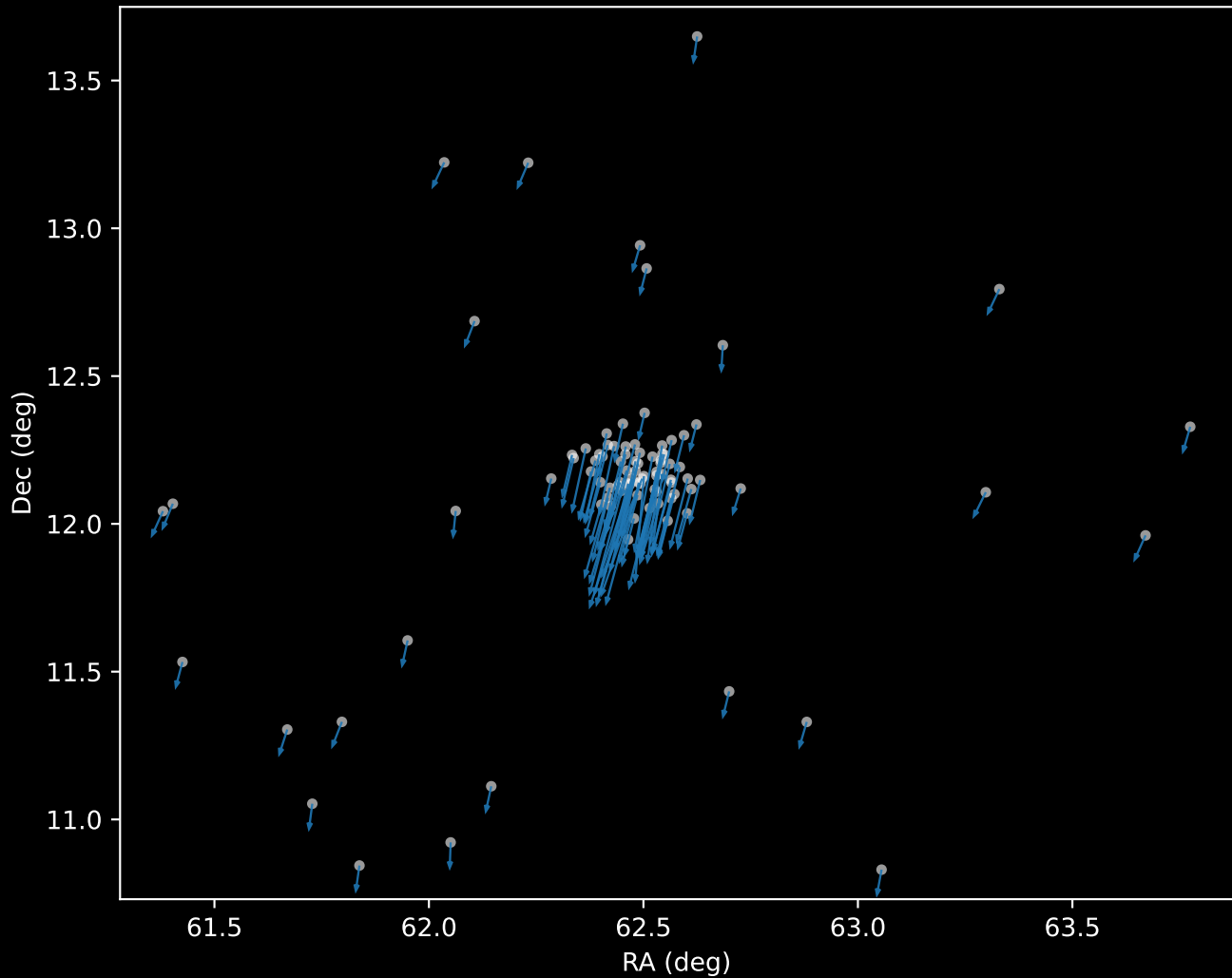
APOGEE DR17 Cluster 40 Proper Motion Vectors (n=93)
