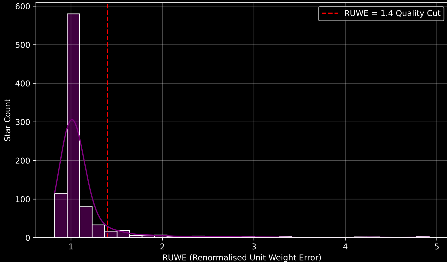
GAPOGEE DR17 Field [M15] RUWE Distribution (n= 899)
