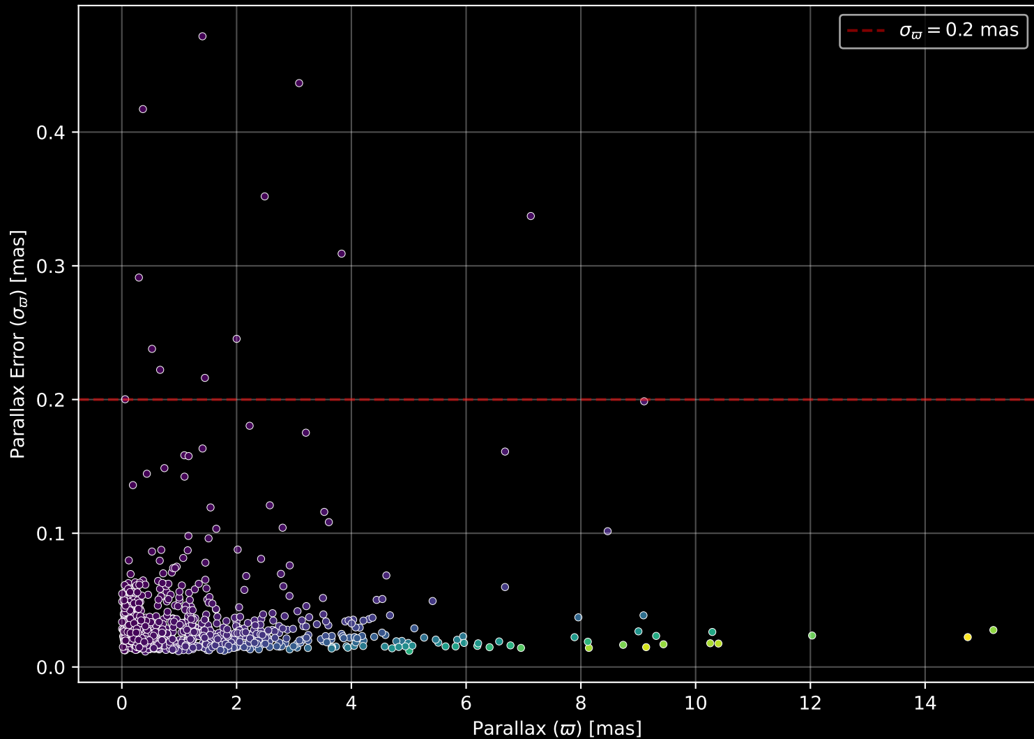
APOGEE DR17 Field: [M15] Parallax Quality (n= 926)
