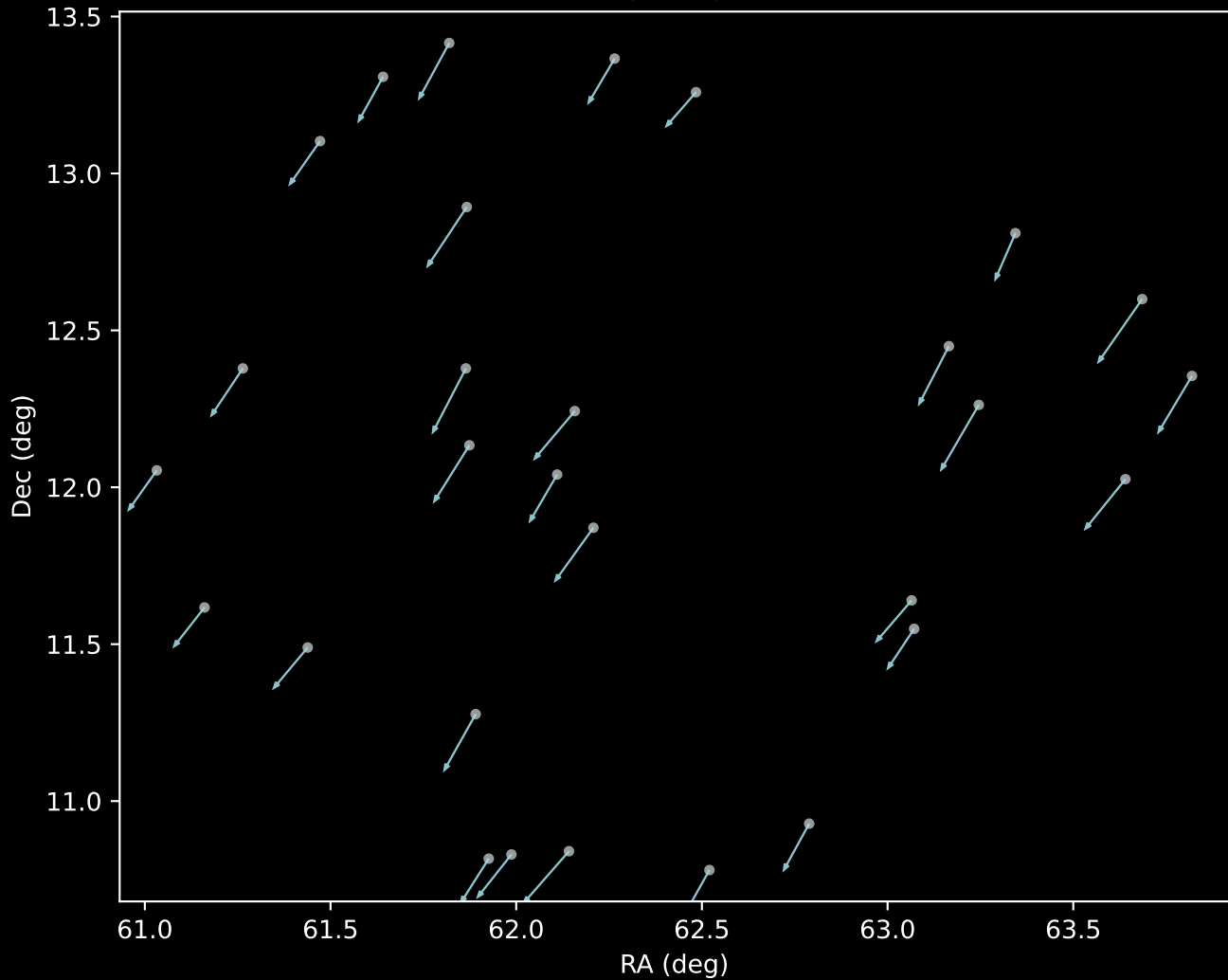
APOGEE DR17 Cluster 39 Proper Motion Vectors (n=29)
