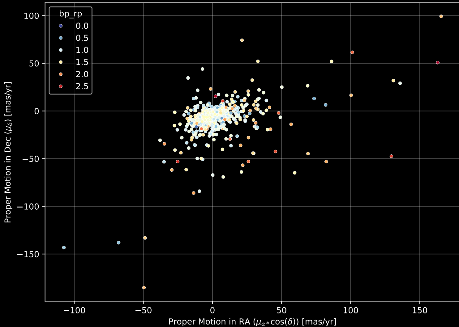
APOGEE DR17 Field: [M15] Proper Motion Diagram (n= 926)
