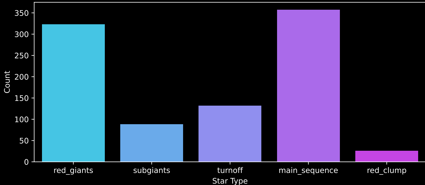
APOGEE DR17 Field: [M15] Count plot of Star Type
