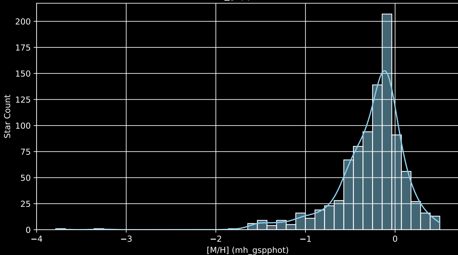
APOGEE DR17 Field: [M15 [M/H] (mh_gspphot) (n= 923)
