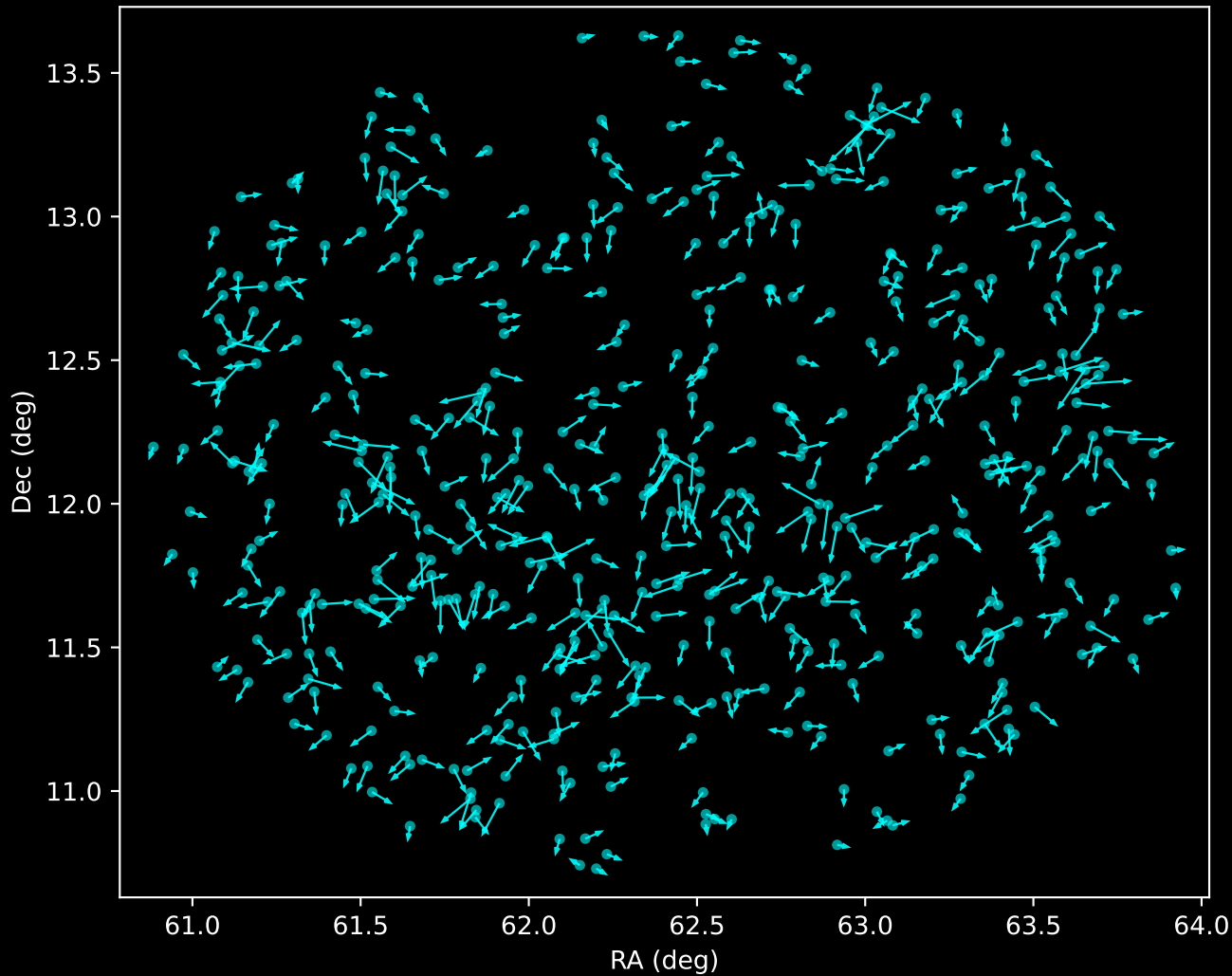
APOGEE DR17 Noise Stream Proper Motion Vectors (n=498)
