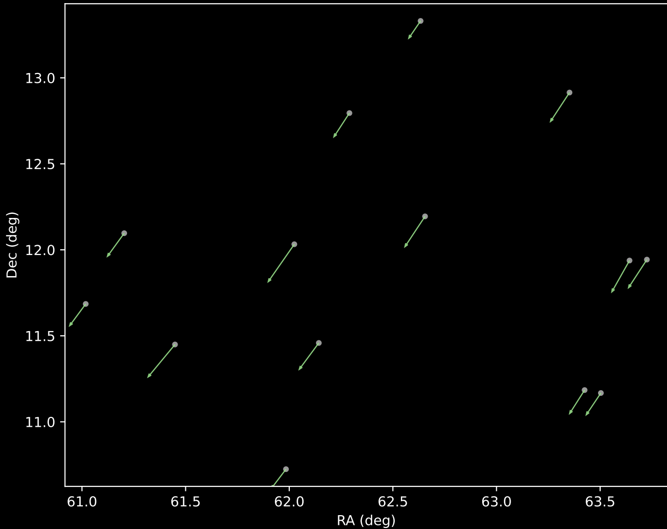
APOGEE DR17 Cluster 25 Proper Motion Vectors (n=14)
